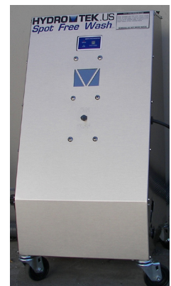
DI water filter cart Connect this DI cart to your existing cold water power washer (up to 3gpm) for spot free washing or connect to a low pressure hose for low flow, unpressurized spot free rinsing. Model# CWD00
